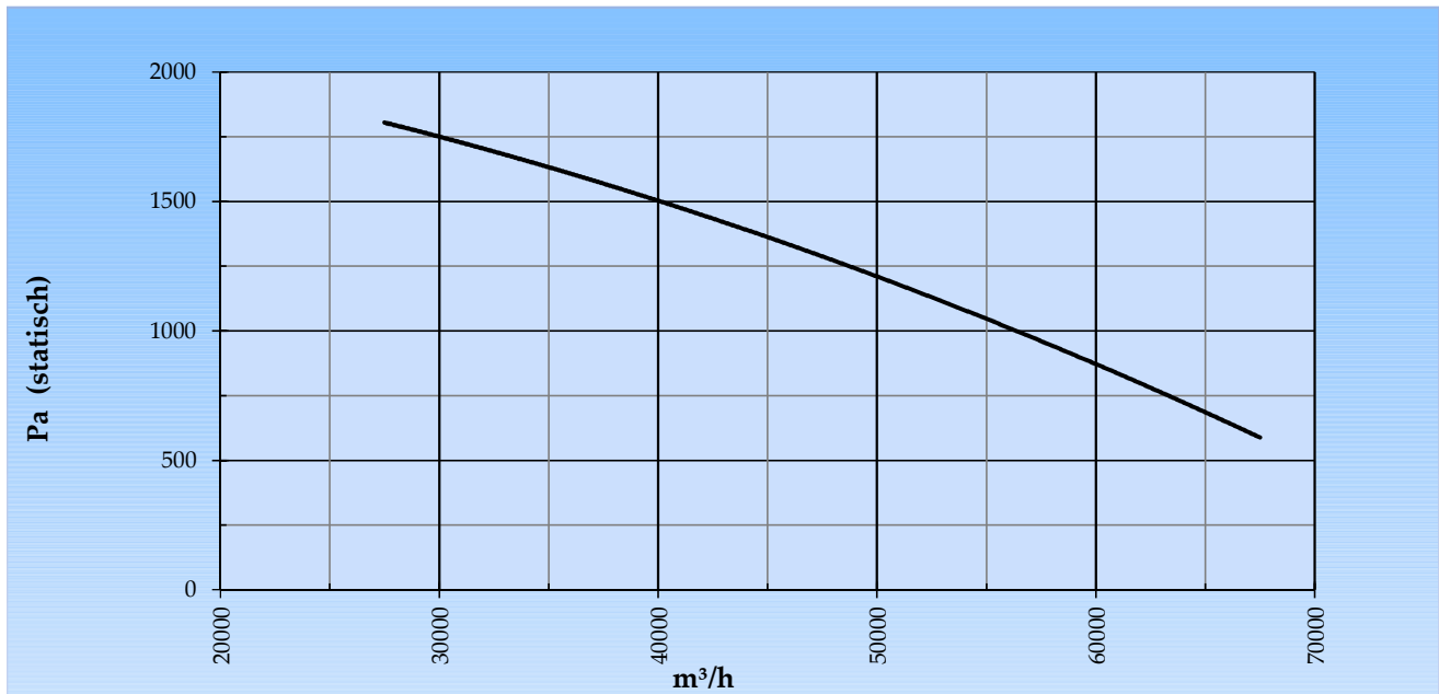
Curve BPR 1122C @ 985rpm @ 15°C @ 0m
